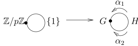
FIGURE 1. Coverings of faithful graphs of groups with universal cover T_{2p}
