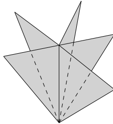
Figure 6: The local picture of an affine building ( n = 2, q = 4 )
