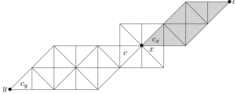
Figure 8: Decomposing into atoms
