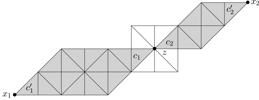
Figure 9: Illustration for Lemma 3.6
