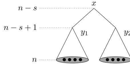
Figure 4: The vertex x has type A.
