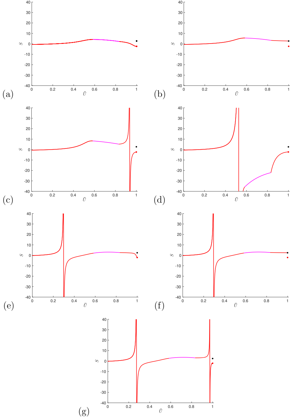
Figure 8: Numerical integration of (98) along \{Y = 0\} for (a) \lambda = 0.1 , (b) \lambda = \lambda_0 = 0 , (c) \lambda = -0.1 , (d) \lambda = -0.3 , (e) \lambda = -0.8 , (f) \lambda = \lambda_1 \approx -0.80925 , (g) \lambda = -0.85 . Red resp. black dots: (projectivisation of) the unstable resp. stable eigenvectors of the saddle-point at \bar{U} = 1 . Magenta segments: concatenated fast jumps defined by the map (90).
