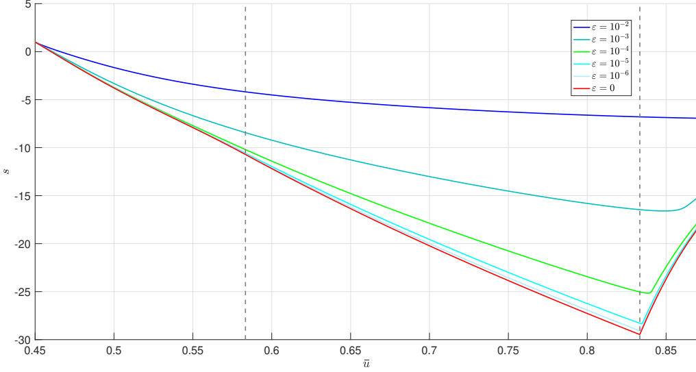
Figure 7: Demonstration of the convergence of the projectivised dynamics (blueish curves) onto the reduced dynamics (red curve) as \varepsilon \rightarrow 0 for \lambda = 15 . Solutions of reduced dynamical system are defined by concatenating the solution of the projectivized flow of dS/d\zeta (see (89)), defined for \bar{U} \in (0, \bar{U}_F) \cup (\bar{U}_J, 1) , with the graph of the map (90) defined for \bar{u} \in [\bar{u}_F, \bar{u}_J] . The left dotted line denotes the fold \bar{u} = \bar{u}_F and the right dotted line denotes the jump curve \bar{u} = \bar{u}_J (and hence the fast dynamics takes place in between these dotted lines). The right dotted line is the jump curve, where the jump condition is used to concatenate the appropriate solutions. The wave speed was held at c = c_0 \approx 0.199362 for each value of \varepsilon .
