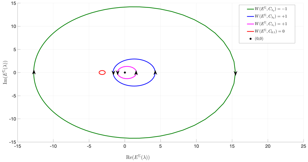
Figure 9: Evaluation of the Riccati-Evans function (109) along circles C_z of radius 0.03 centered at the point z \in \mathbb{C} . The winding numbers along each contour are given in the legend and are also depicted by the arrowheads. Note that \lambda_0 and \lambda_1 denote the two eigenvalues and \lambda_p = -0.08 is the approximate location of the pole of E^\Sigma(\lambda) .
