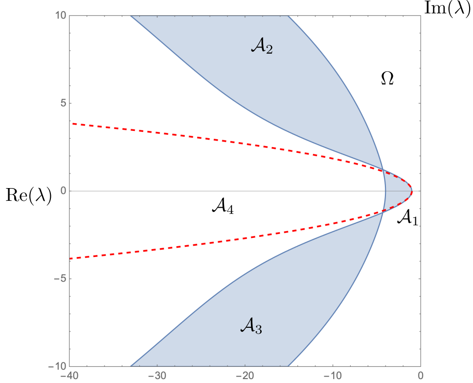
Figure 10: Plot of the essential spectrum (shaded regions) of the of the linearised operator L in (112), which shows \Omega and the \mathcal{A}_i partitioning the complex plane via the Fredholm borders (continuous spectrum). The shape of the essential spectrum means that the operator L , for non-zero \varepsilon is sectorial. The dashed line (red online) is one of the Fredholm borders coming from the linearisation of the reduced problem about the (constant) steady-state \bar{U}^- c.f. the right figure in Fig 4. For the figure, \varepsilon = 0.1 and c = a = 1 , with D and R as in (3) and (4).
