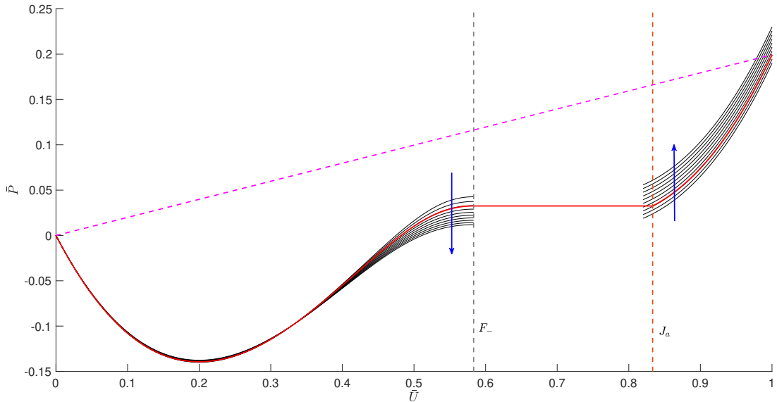
Figure 2: Segments of W^u(\bar{Z}^-) and W^s(\bar{Z}^+) arising from the slow flow (19)–(20), as c is varied within the range [0.19, 0.23] . The stable manifolds are extended slightly past J_a to illustrate the transversality of the slow flow at J_a . The singular homoclinic orbit \Gamma_0 is depicted by the red curve for c_0 \approx 0.199362 . The blue arrows indicate how the (un)stable manifolds vary as c is increased. The magenta dashed line denotes the \bar{U} -nullcline for c = c_0 .
