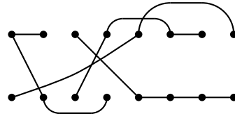
Figure 1: A graphical representation of a block bijection \theta \in \mathcal{S}_8^* .
