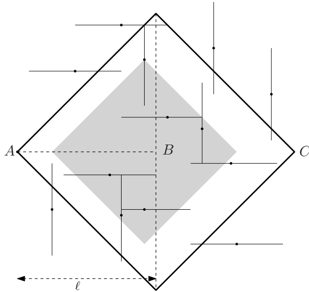
FIGURE 4. Only seeds within the large square (whose diagonal is AC ) can influence the event that an H -type ray starting at A does not reach B (due to intersection of the line-segment AB by vertical rays). The role of the smaller shaded square is described in the text.
