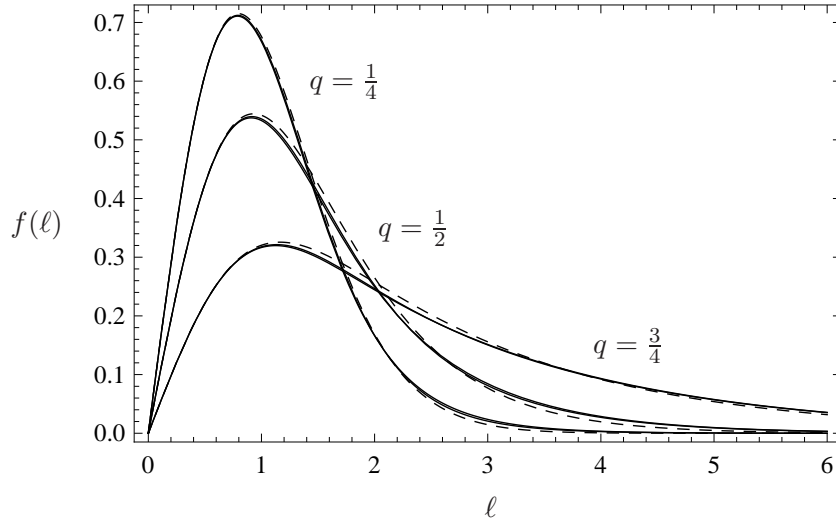
FIGURE 3. The three solid curves are the probability density functions f for the final length of a typical eastward-growing ray in the half-Gilbert model. Each is based on \lambda = 2 and with three q values: \frac{1}{4} , \frac{1}{2} and \frac{3}{4} . We show later in the paper that: (a) each of these solid curves actually comprises two curves overlaid, the second being the curve from the full-Gilbert model, with \lambda = 1 ; (b) the dashed lines are the probability density functions from Gilbert's heuristic 'mean field' analysis, also valid for both models.
