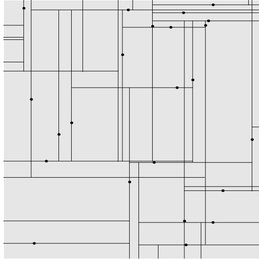
FIGURE 1. A realisation of the rectangular tessellation (discussed by Cowan and Ma) for the balanced case when V -type and H -type seeds have equal intensities. A realisation of the full Gilbert model having rectangular cells can be found in Figure 11 of [7].
